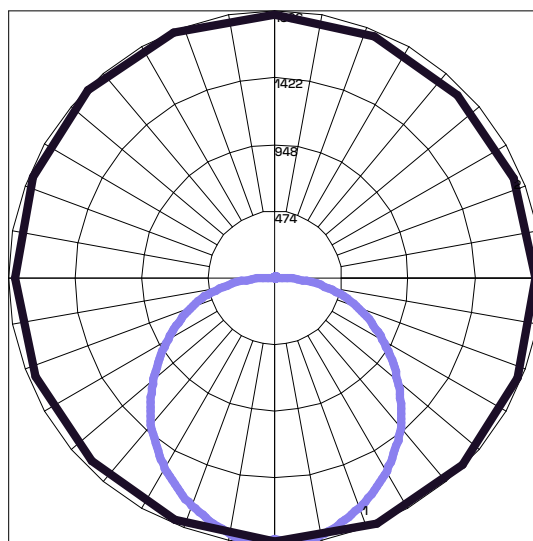
Maximum Candela = 1896.2 Located At Horizontal Angle = 292.5, Vertical Angle = 5 # 1 - Vertical Plane Through Horizontal Angles (292.5 - 112.5) (Through Max. Cd.) # 2 - Horizontal Cone Through Vertical Angle (5) (Through Max. Cd.)
