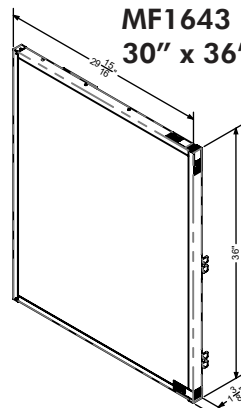
Single Face Light Box
